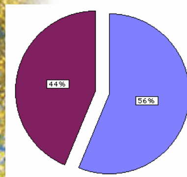
Emission to Air - Textil Industry - (2006)
