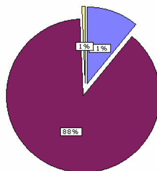
Emission to Air - Waste management (2006)
